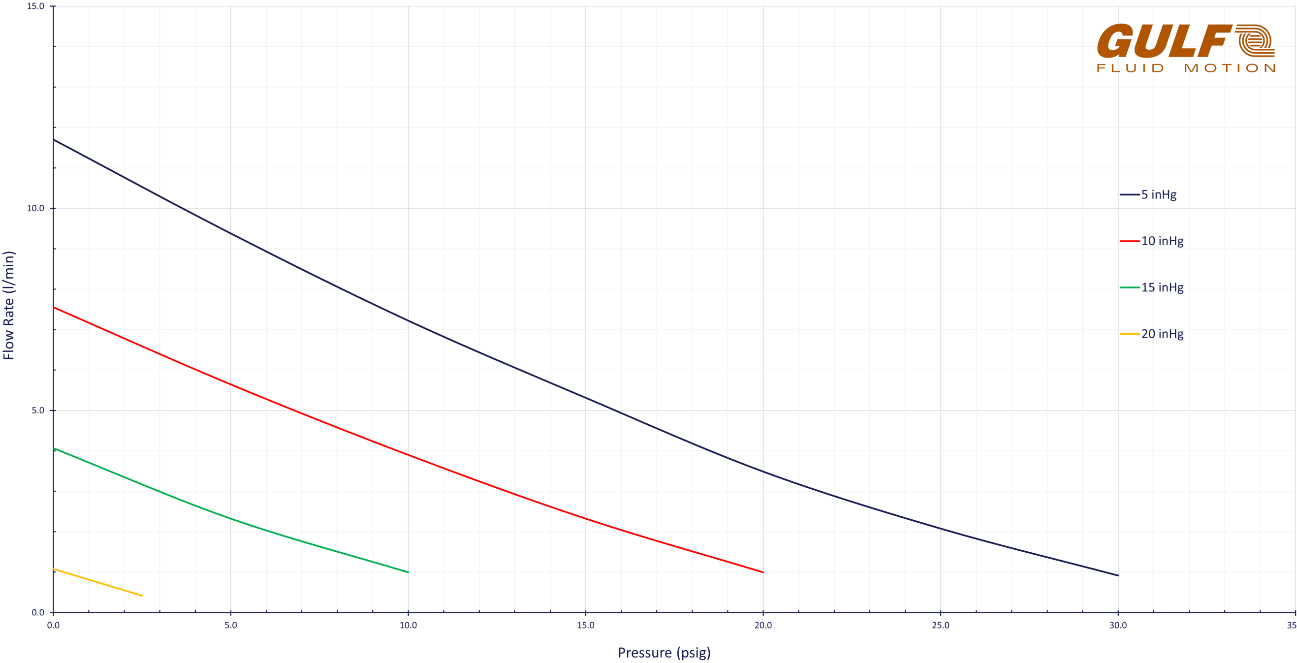
Combination Curves - 400 Series Single Head - High (50Hz)
