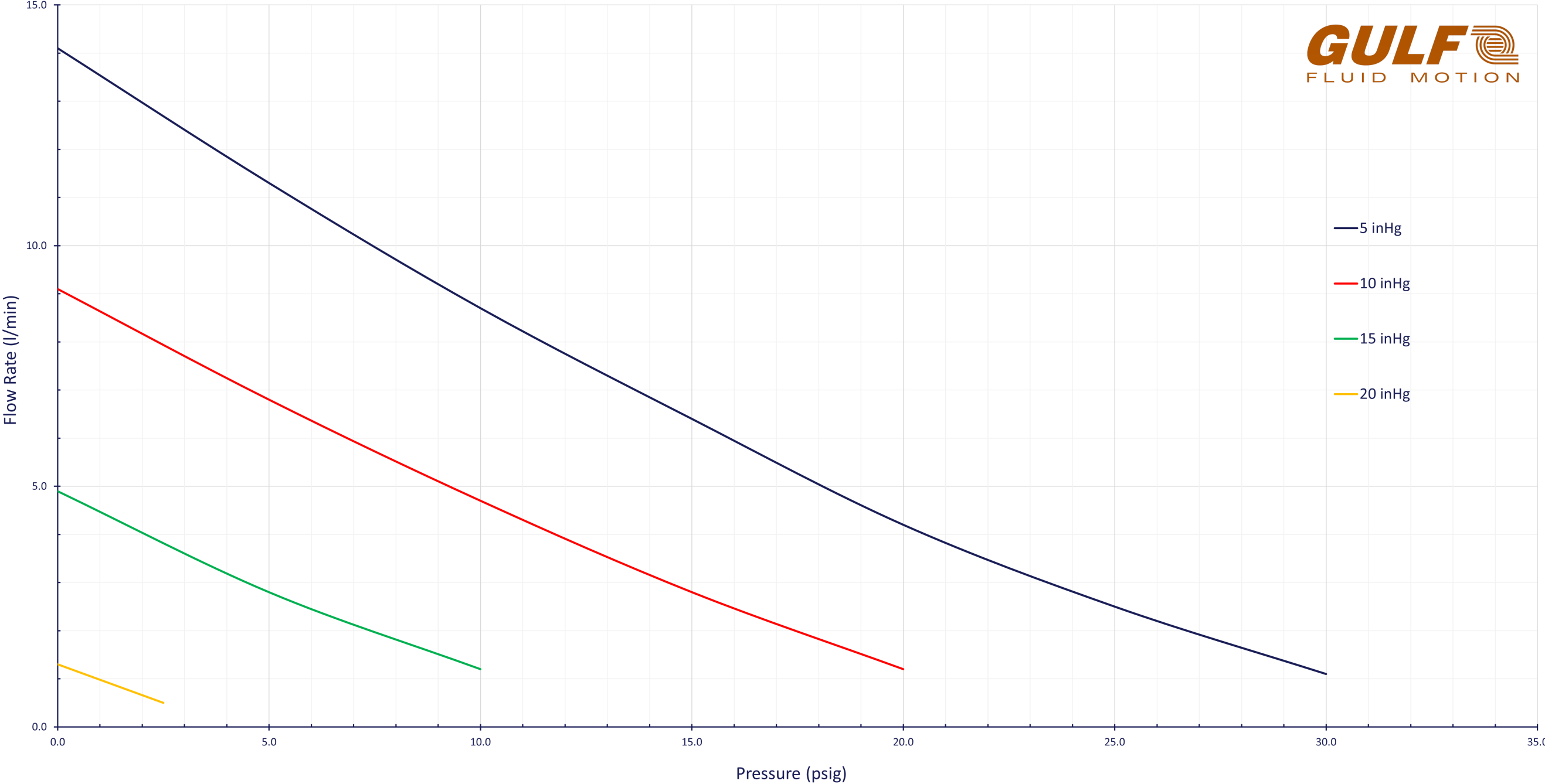
Combination Curves - 400 Series Single Head - High (60Hz)
