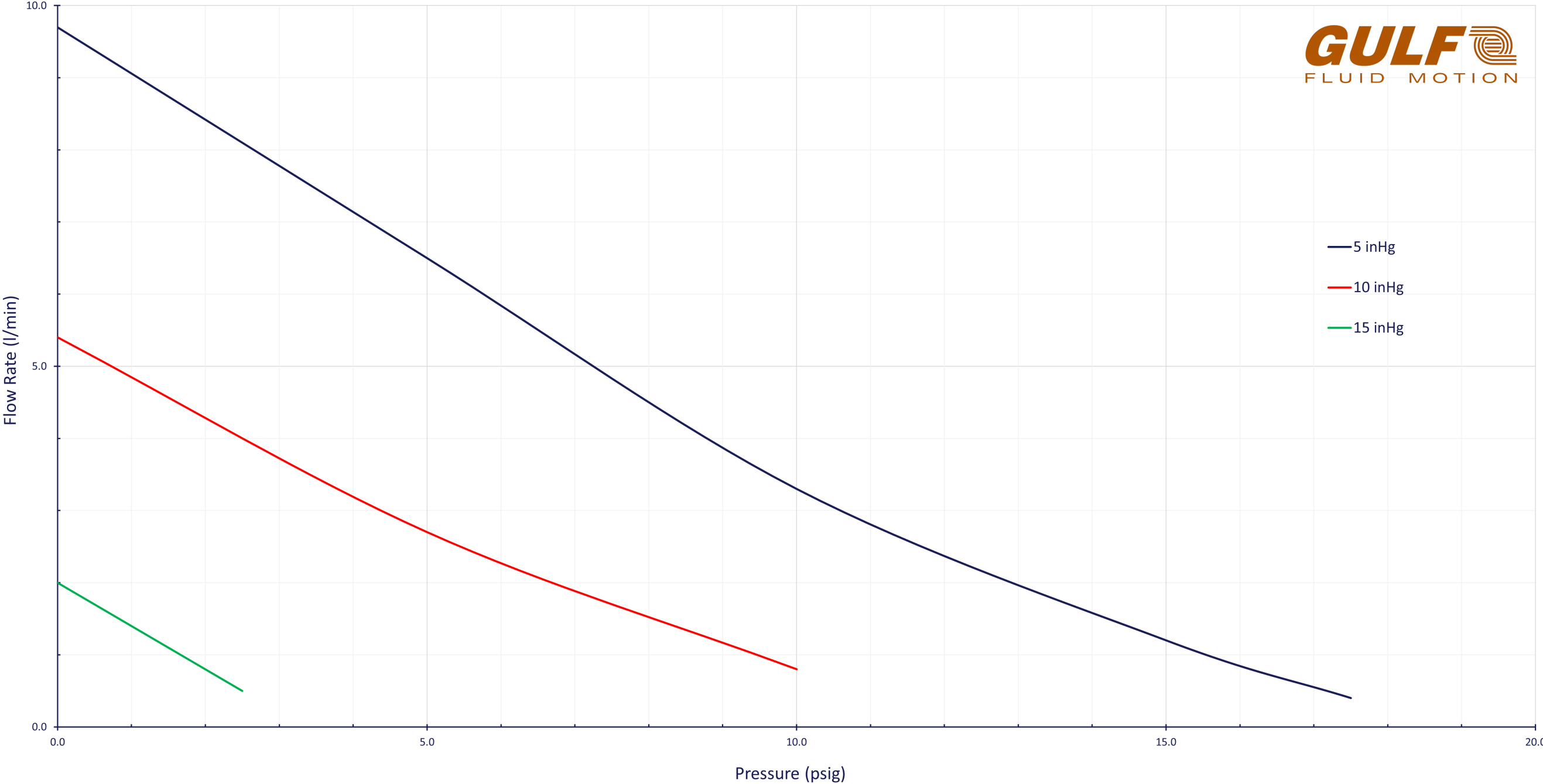
Combination Curves - 400 Series Single Head - Low (60Hz)
