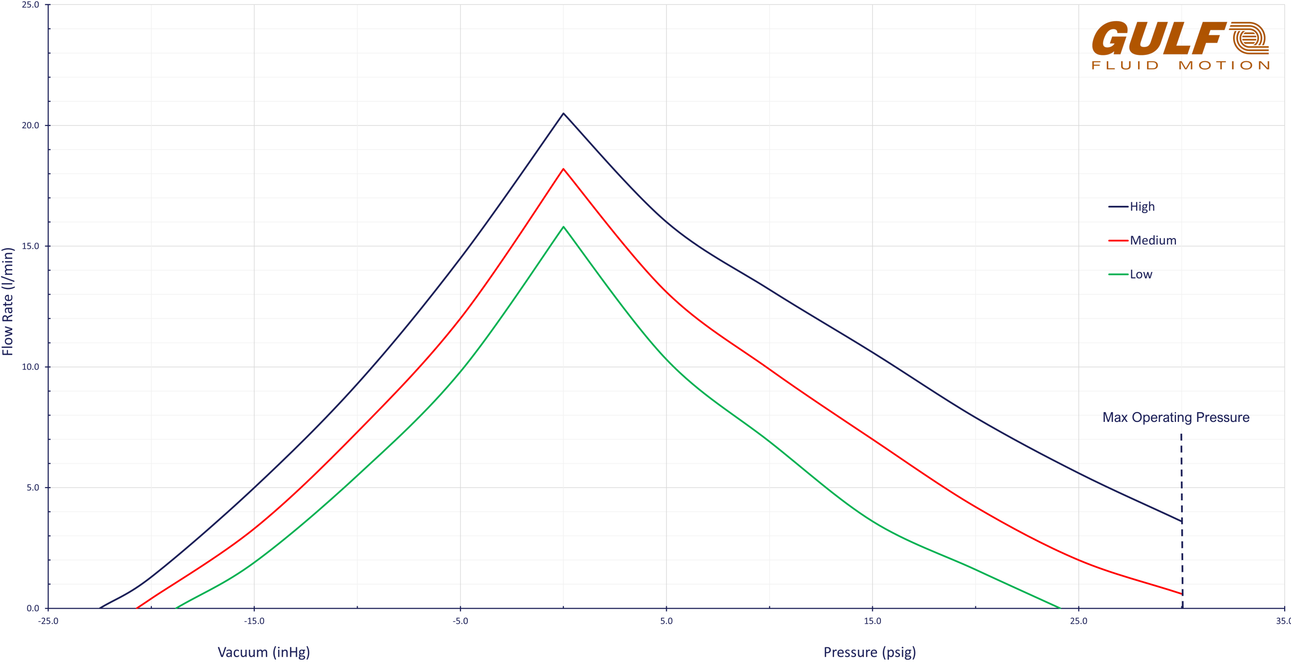
Performance Curves - 400 Series Single Head (60Hz)
