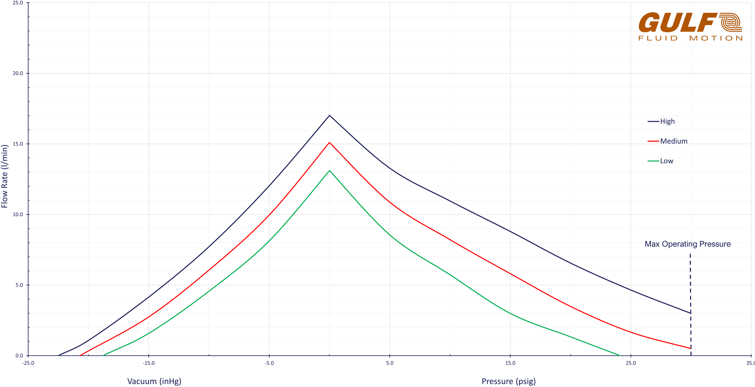
Performance Curves - 400 Series Single Head (50Hz)
