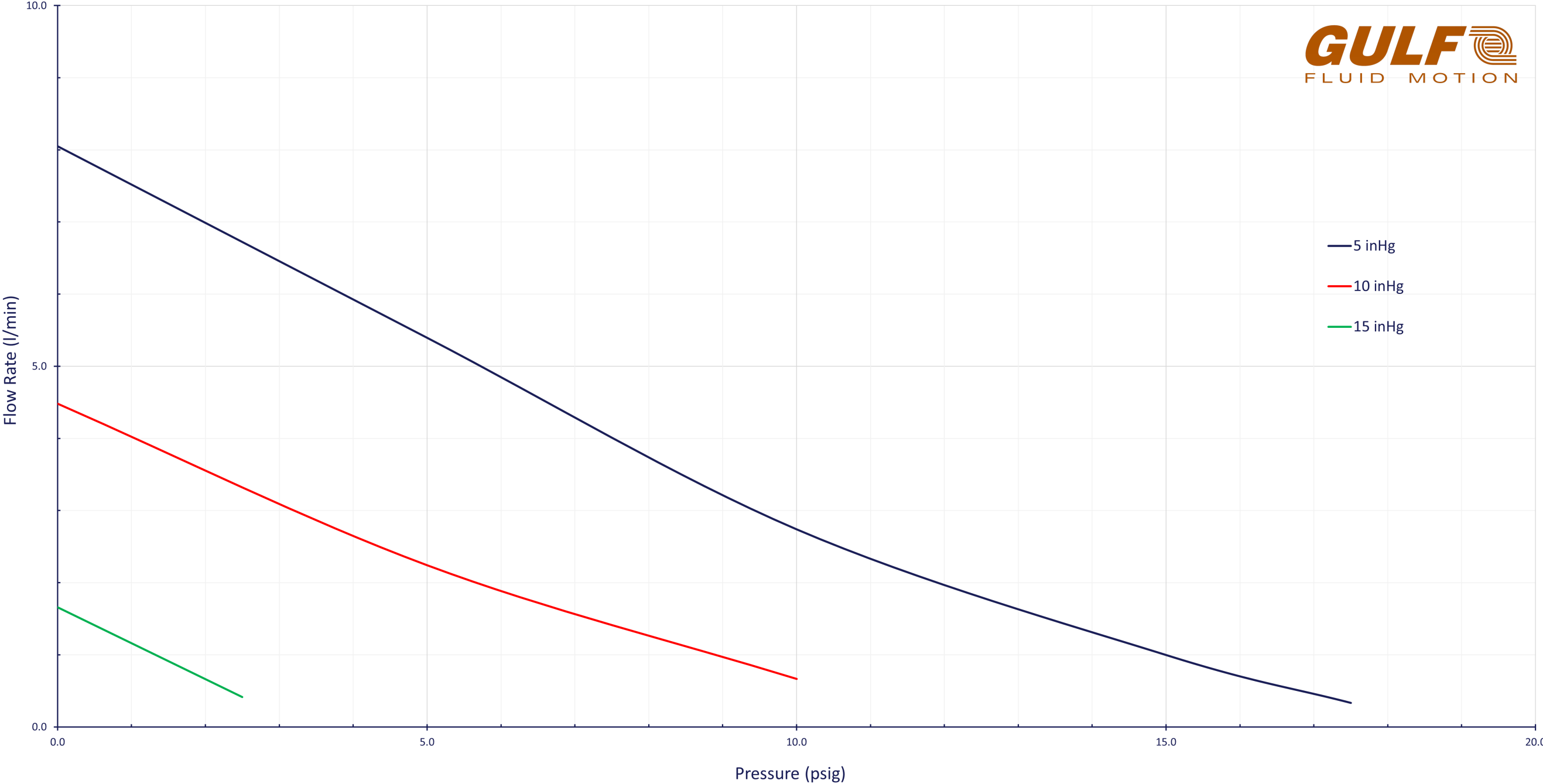
Combination Curves - 400 Series Single Head - Low (50Hz)
